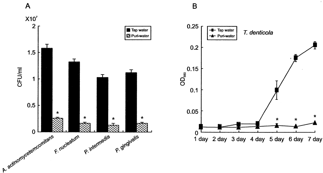
Fig. 2. Bacteria in wash solution of toothbrushes with Puri-water. Toothbrushes were contaminated with periodontopathogens ( OD_{660} = 0.5 ), and washed with Puri-water or tap water. CFU was counted on BHI agar medium (A) or OD 660 was measured in OMIZ-Pat broth medium (B) after culturing the wash solution. For each bacterium, seven brushes were used and the experiments were repeated three times. *Significant difference ( P < 0.05 ) compared to the values that were obtained after exposure to tap water.
